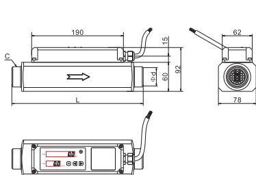
(图5-1) MF2025/MF2032 BSPT接口外形尺寸
